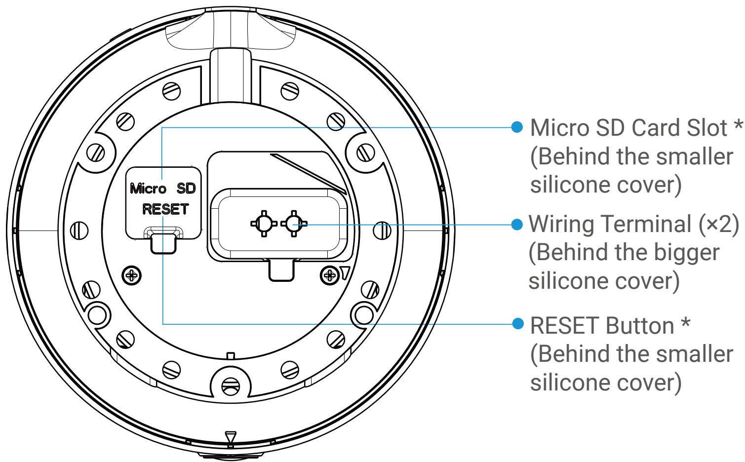
Bottom View
